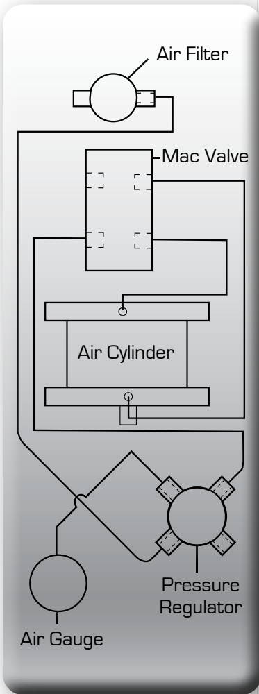
Air Line Diagram
